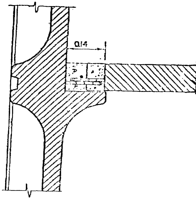
JUNTA HORIZONTAL LOSA ENTREPISO- PANEL VERTICAL
